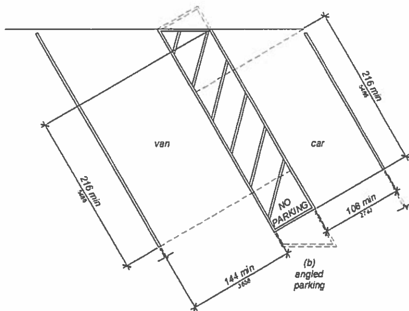
FIGURE 11B-502.2 VEHICLE PARKING SPACES
