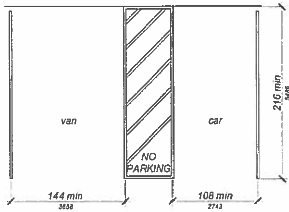
(a) perpendicular parking
