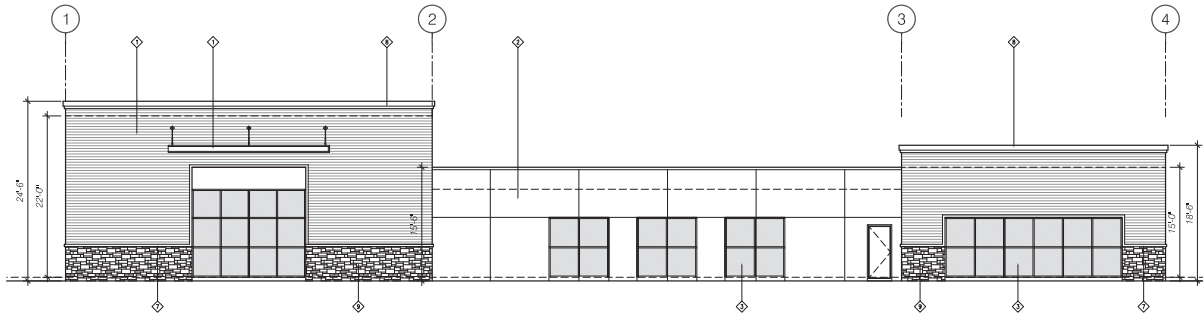
3 SOUTH ELEVATION SCALE : 1/8"=1'-0"
