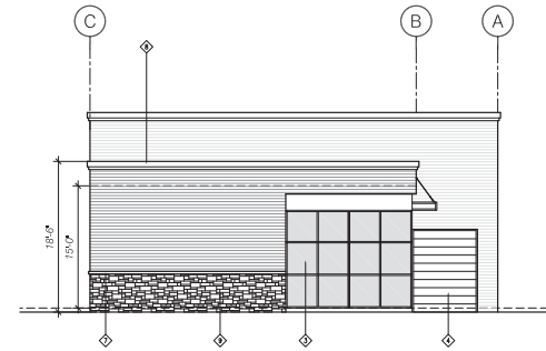
1 EAST ELEVATION SCALE : 1/8"=1'-0"
