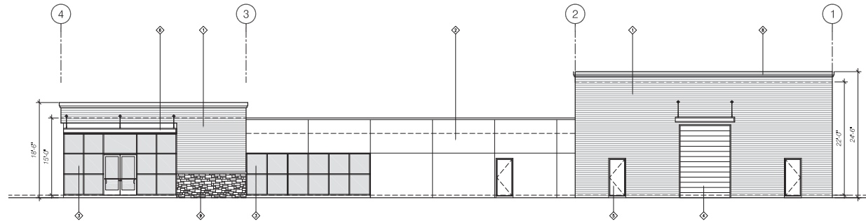
2 NORTH ELEVATION SCALE : 1/8"=1'-0"
