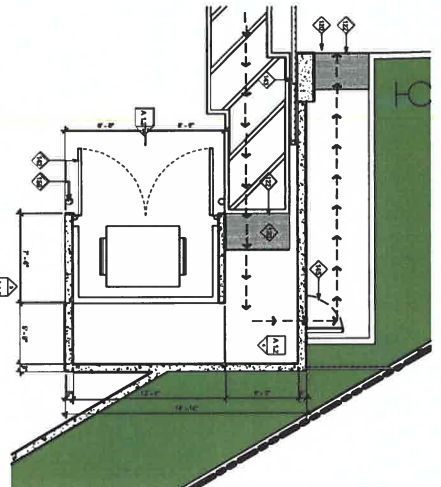
1 ENLARGED TRASH ENCLOSURE PLAN 1/8" = 1'-0"
