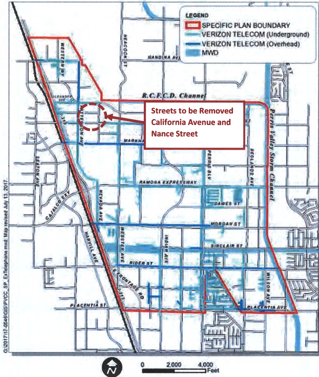
Figure 3.0-14, Existing Telephone
