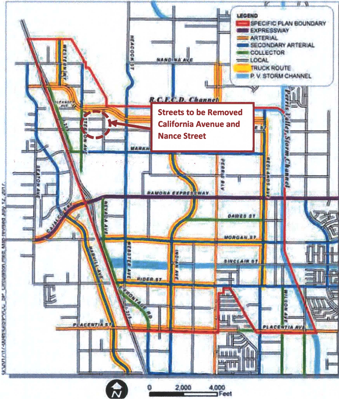
Figure 3.0-1, Circulation Plan
