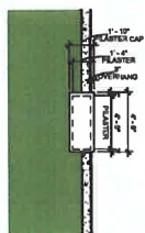
11 TYPICAL PLASTER CAP PLAN 1/8" = 1'-0"
