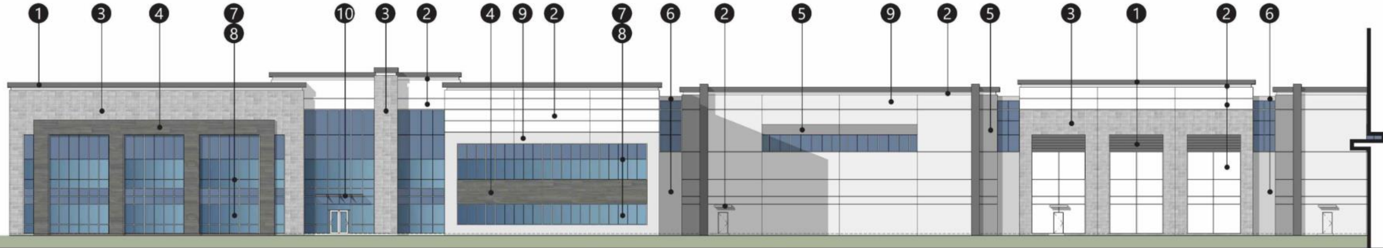
Enlarged View of South Elevation
