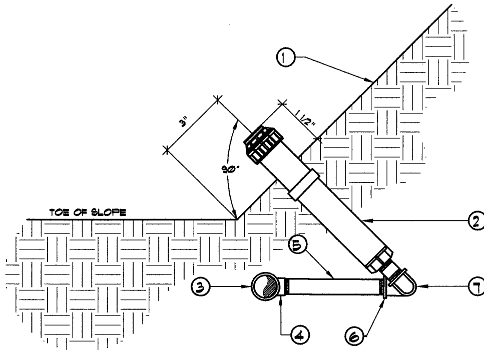
(TRIPLE SWING ASSEMBLY)
