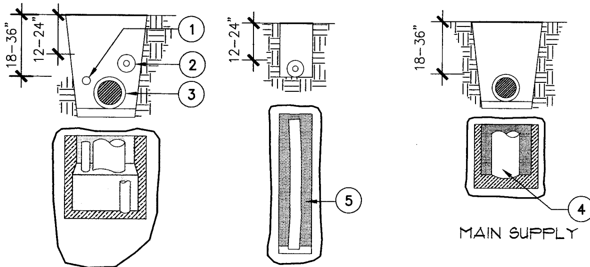
MAIN SUPPLY, LATERAL, & WIRING LATERAL
